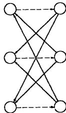
Figure 2. Solution for 3-fence inequality.
