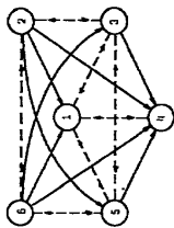
Figure 4. Fractional solution of Problem 6.
