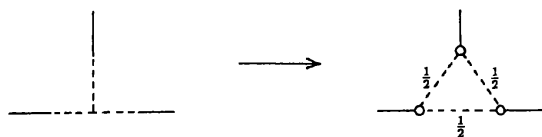
Figure 5. Model of a three-way junction in a layout graph.
